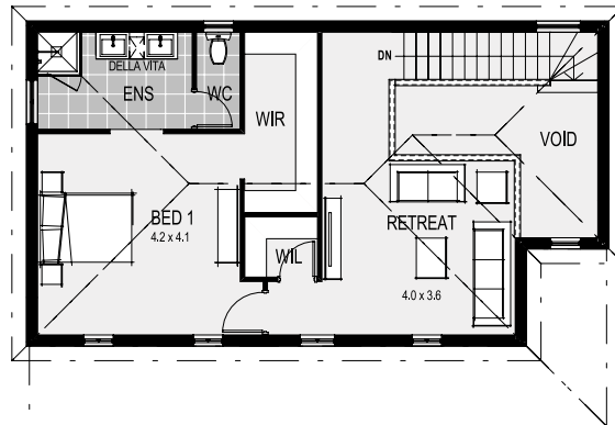
UPPER FLOOR 1:100
