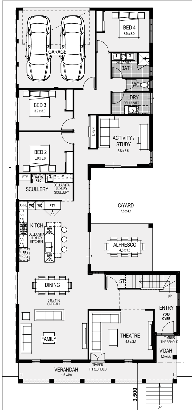
GROUND FLOOR 1:100
