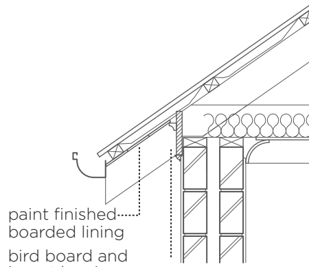
Raked and Lined Eaves
