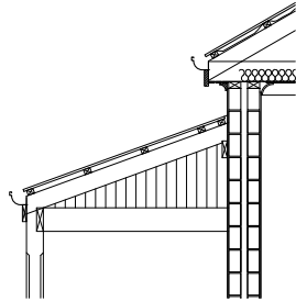
Straight Verandah
