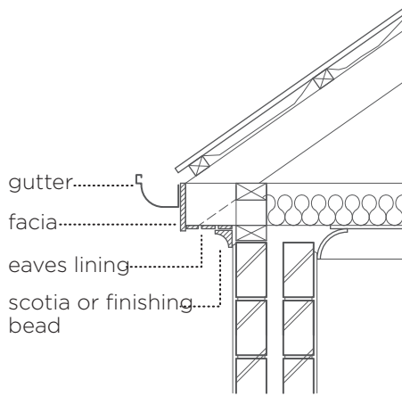
Traditional (Boxed) Eaves
